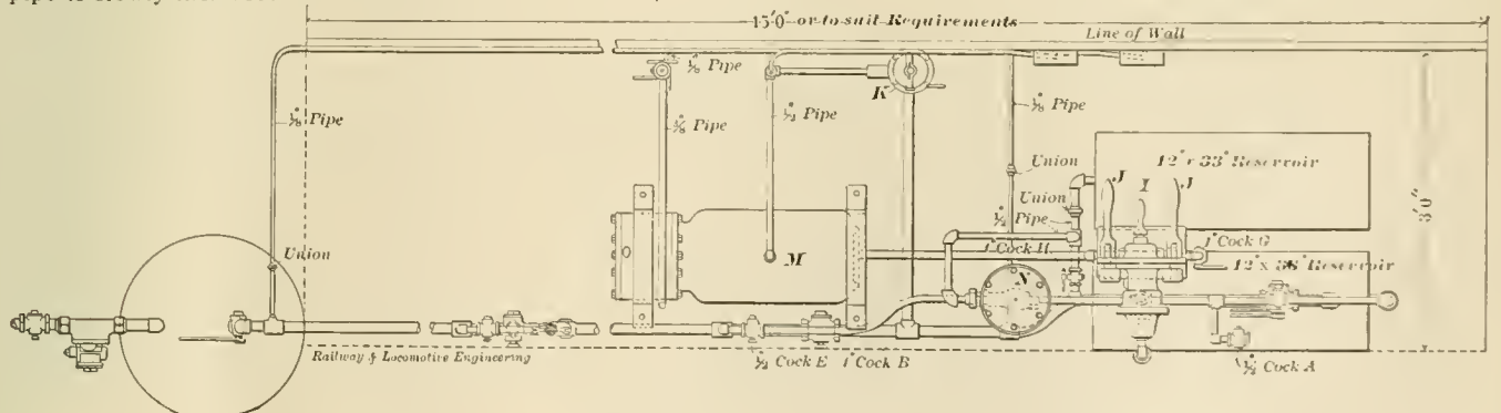
SHOP TEST RACK FOR REPAIRED TRIPLES—TOP VIEW.
